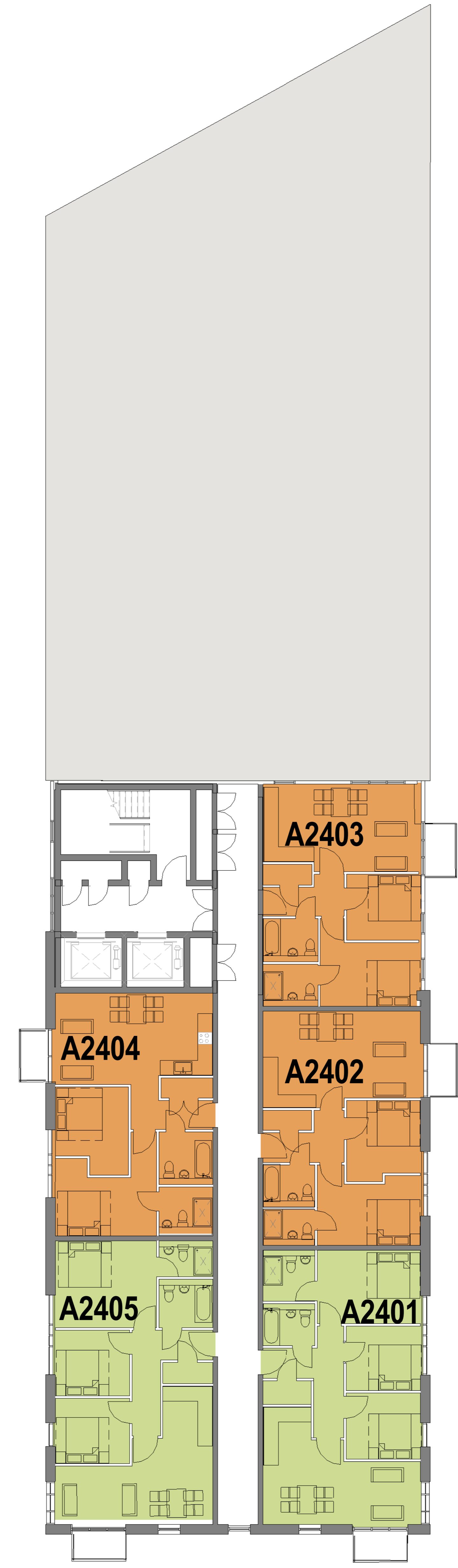
1 Block A - Twenty Fourth Floor 1:100
